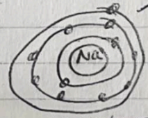
11 electrons
